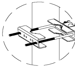
Fix bottom Clip brackets on mounting pipe.
